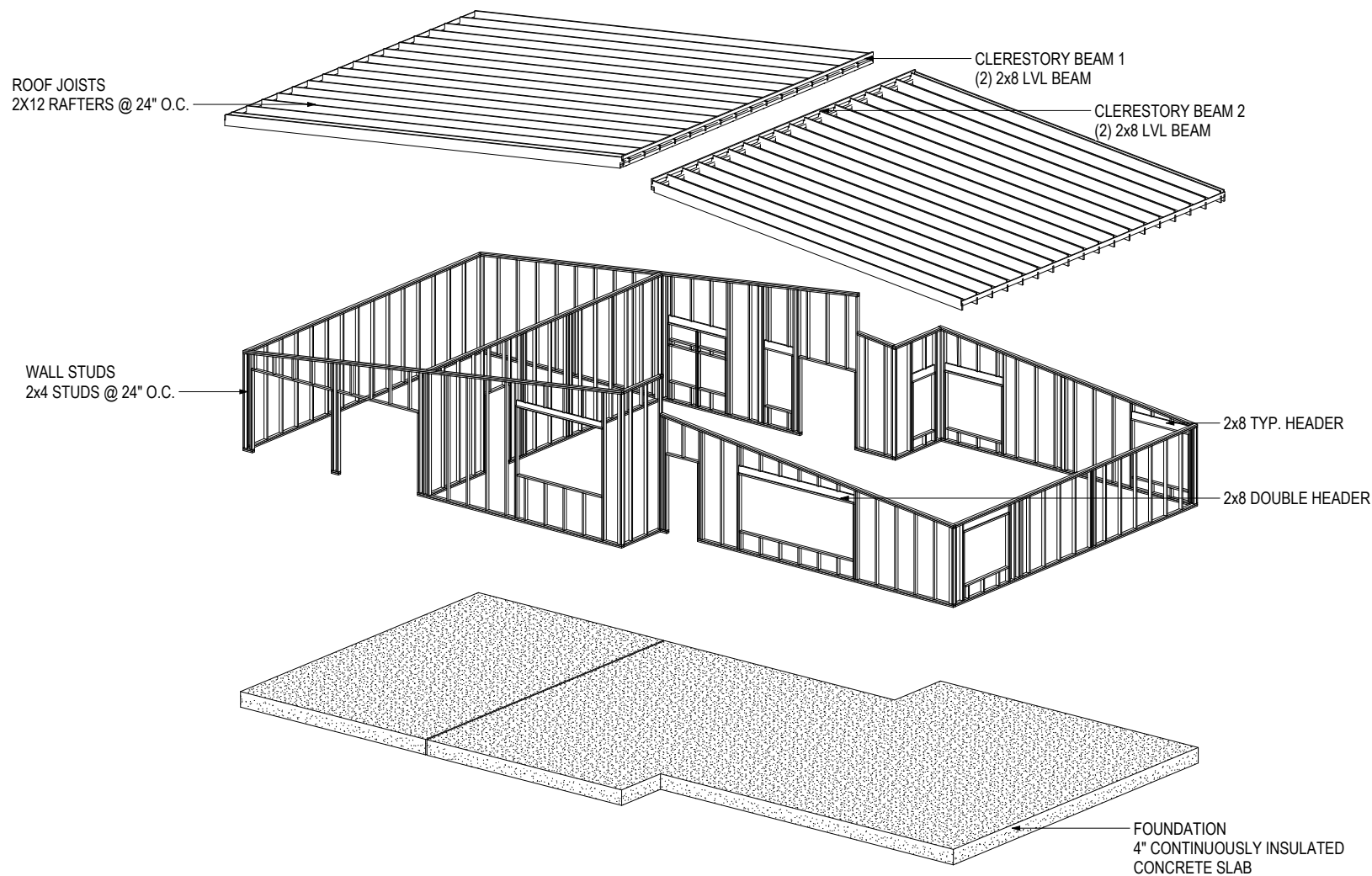
STRUCTURAL DIAGRAM
