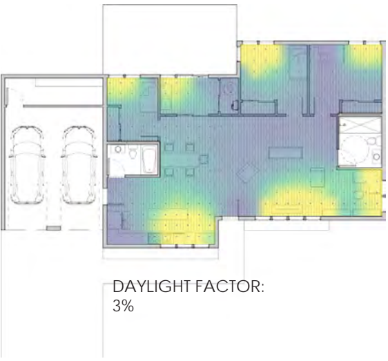
DAYLIGHT ANALYSIS
